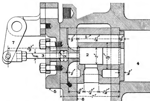
Fig. 2209. Starting Valve for Cole Four-Cylinder Balanced Compound Locomotive.
